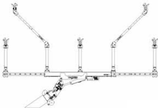
Horizontal Configuration with Dual Monopole Static Arm Attachment
