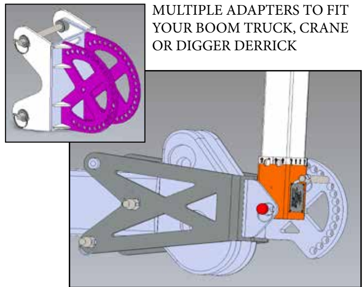
TOOL-LESS MAST INSTALLATION AND ANGLE ADJUSTMENT
